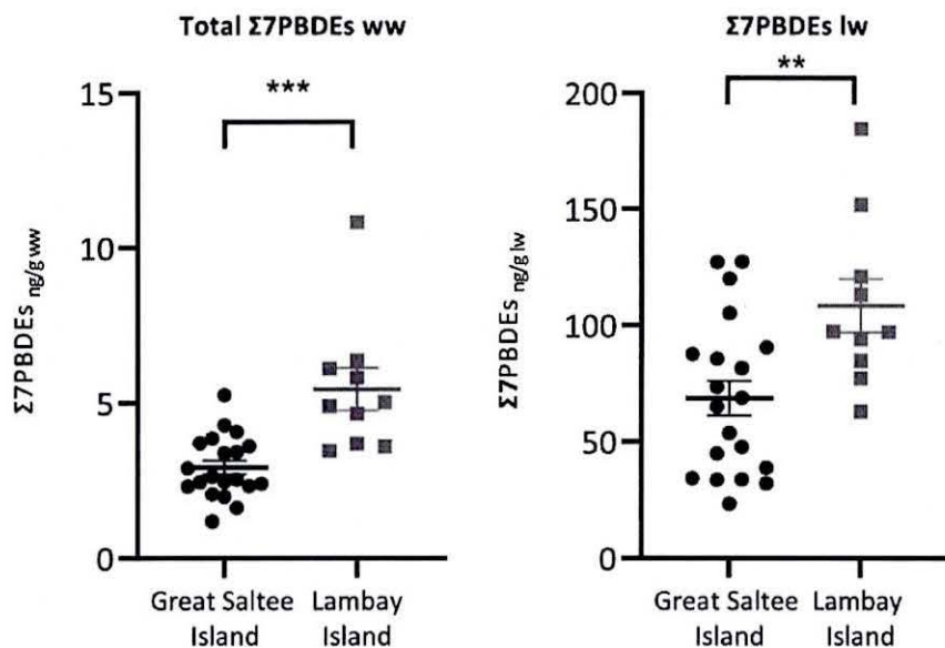
Fig. 3. \Sigma 7PBDE ng/g ww and lw concentrations in Gannet eggs in Great Saltee Island (n = 20) and Lambay Island (n = 10), statistical significance was tested by Mann Whitney test for ww (non parametric data) and by unpaired t-test for lw (parametric). Error bars = SEM, ** = P \leq 0.01 *** = P \leq 0.001 .
